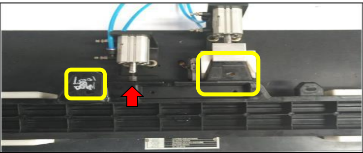
POKA – YOKE FOR SPRING NUT MISSING
